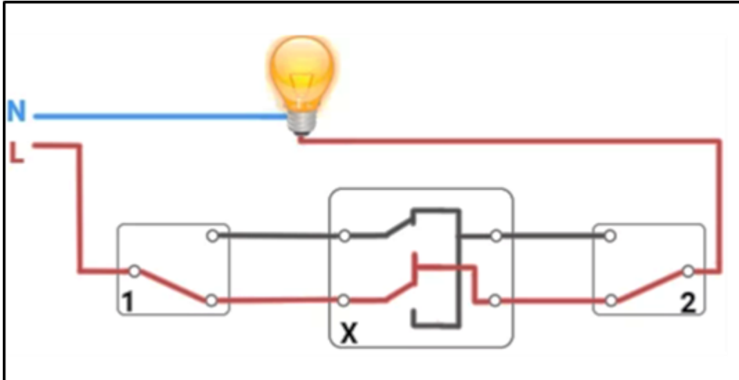
Figure 4.7. Crossover switch wiring diagram
