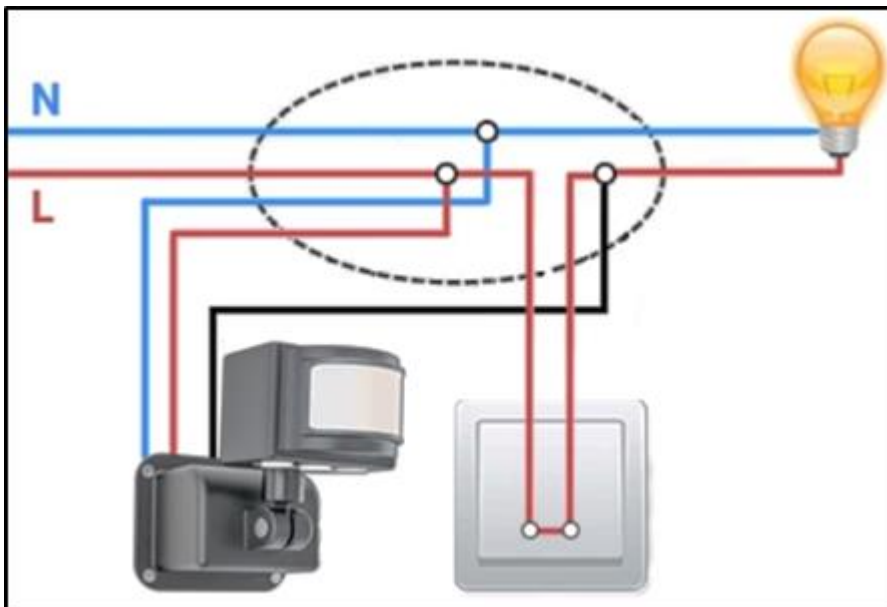
Figure 4.8. Switch with infrared sensor
